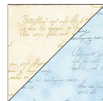
ninety J/K HSTs
